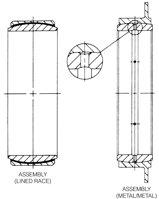
FIGURE 11 - SNAP-ASSEMBLED BEARINGS
