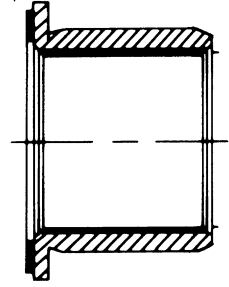
FIGURE 13 - FLANGE, TEFLON LINED
